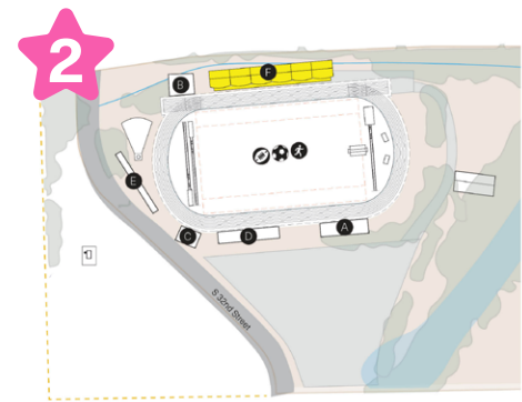
7 BUILD NEW 2500 BLEACHER F WITH SHADING
